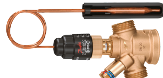
PICV+QT: AB-QT
