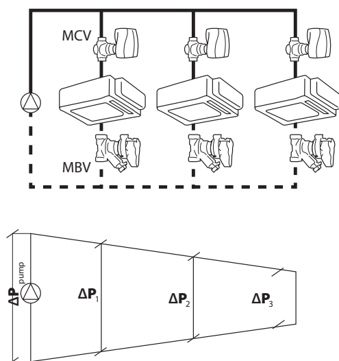
Fig 10.1 Direct return system (not recommended system)
