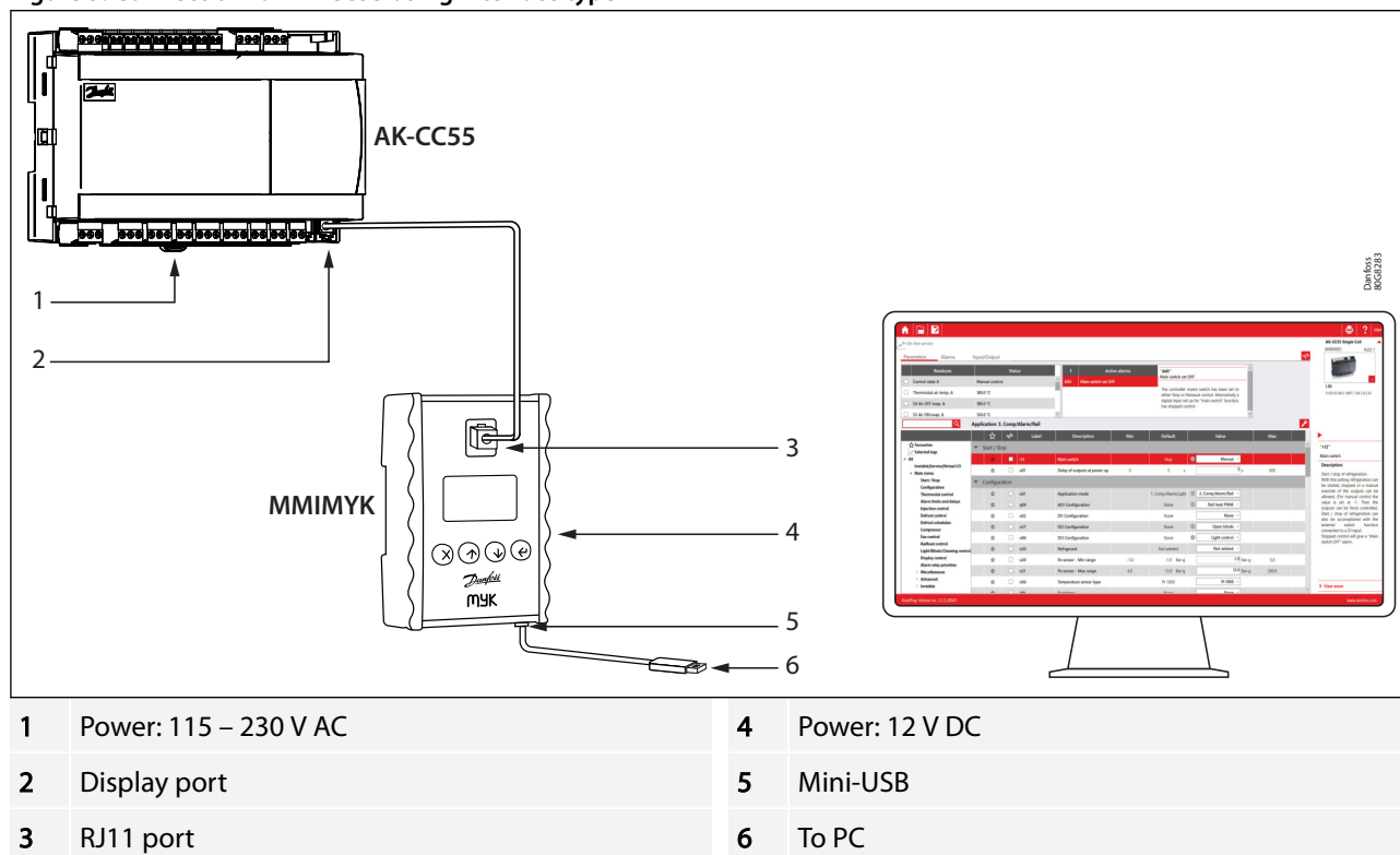
Figure 5: Connection for AK-CC55 using interface type MMIMYK
