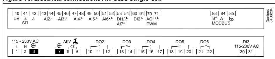
Figure 16: Electrical connections AK-CC55 Single Coil
