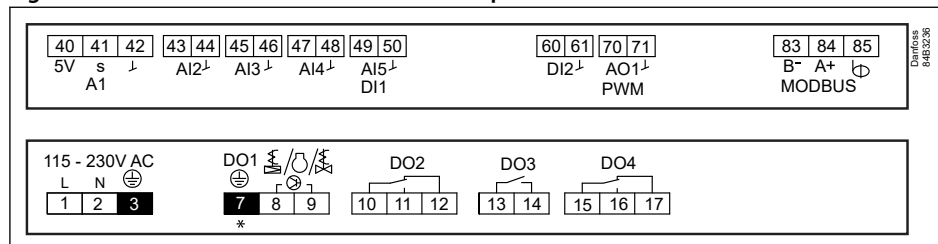
Figure 15: Electrical connections AK-CC55 Compact
