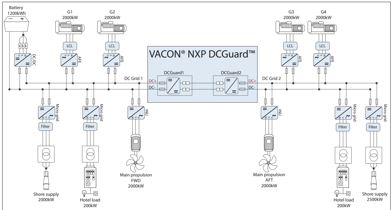
Figure 2 Wiring diagram of a DC grid illustrating VACON® NXP DCGuard™.
