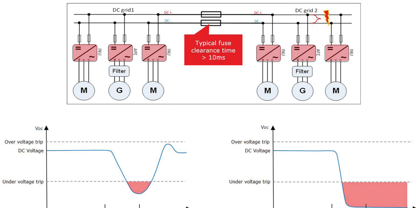
Figure 1 Long fuse clearance time in a DC grid results in a blackout.
