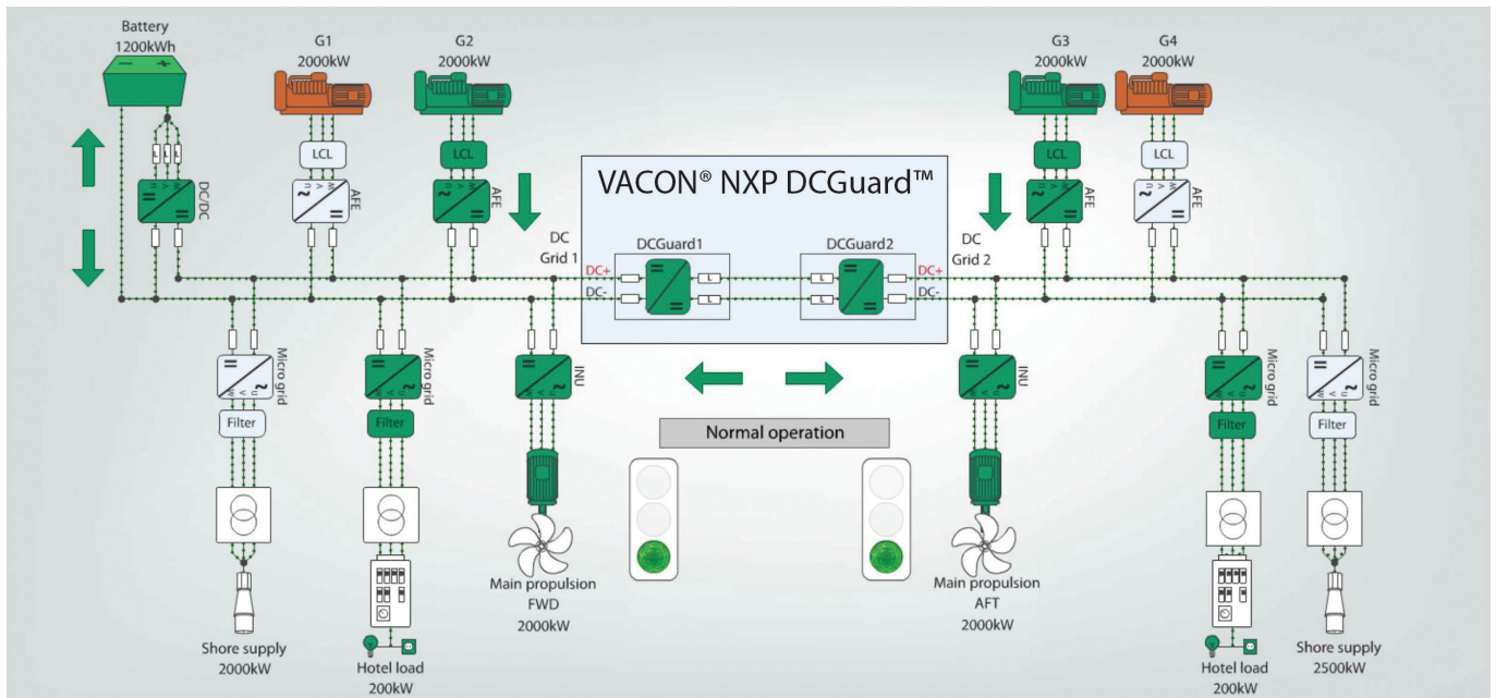
Figure 3 Normal operation.
