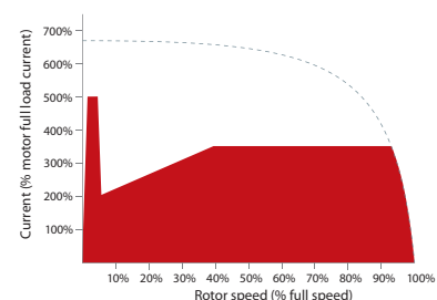
Constant current/current ramp – here shown with kickstart
