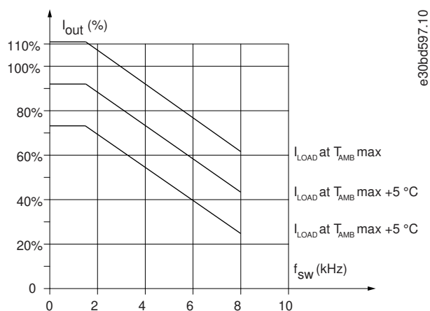
Illustration 94: Output Current Derating with Switching Frequency and Ambient Temperature for Enclosure Size C3
