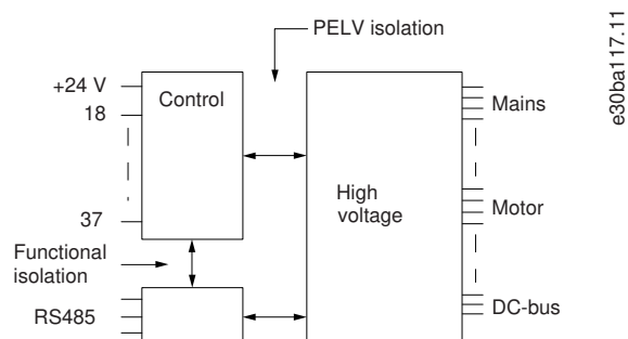
Illustration 52: PELV Isolation
