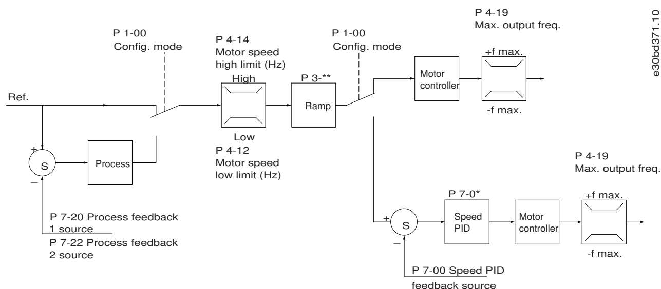
Illustration 149: Control Structure in VVC+ Open-loop Configurations and Closed-loop Configurations
