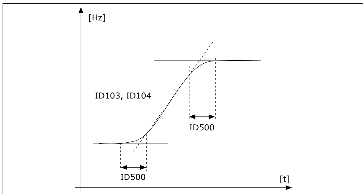
Fig. 48: Accelerations/decelerationskurven (S-formet)
