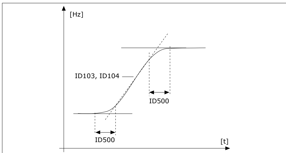
Fig. 49: Accelerations/decelerationskurven (S-formet)
