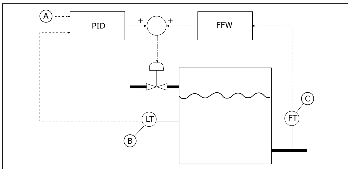
Fig. 80: Feedforward-styring
