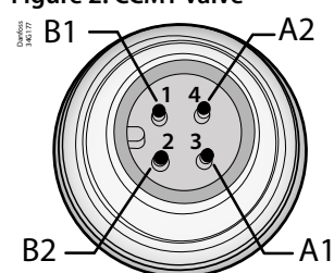
Figure 2: CCMT valve
