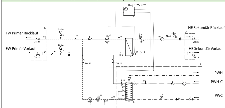
HYDRAULIKSCHEMA - TERMIX COMPACT 28 VX-FI HWP; AVQM
