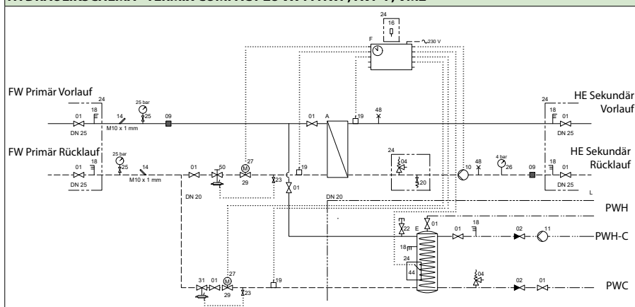
HYDRAULIKSCHEMA - TERMIX COMPACT 28 VX-FI HWP; AVP-F; VM2
