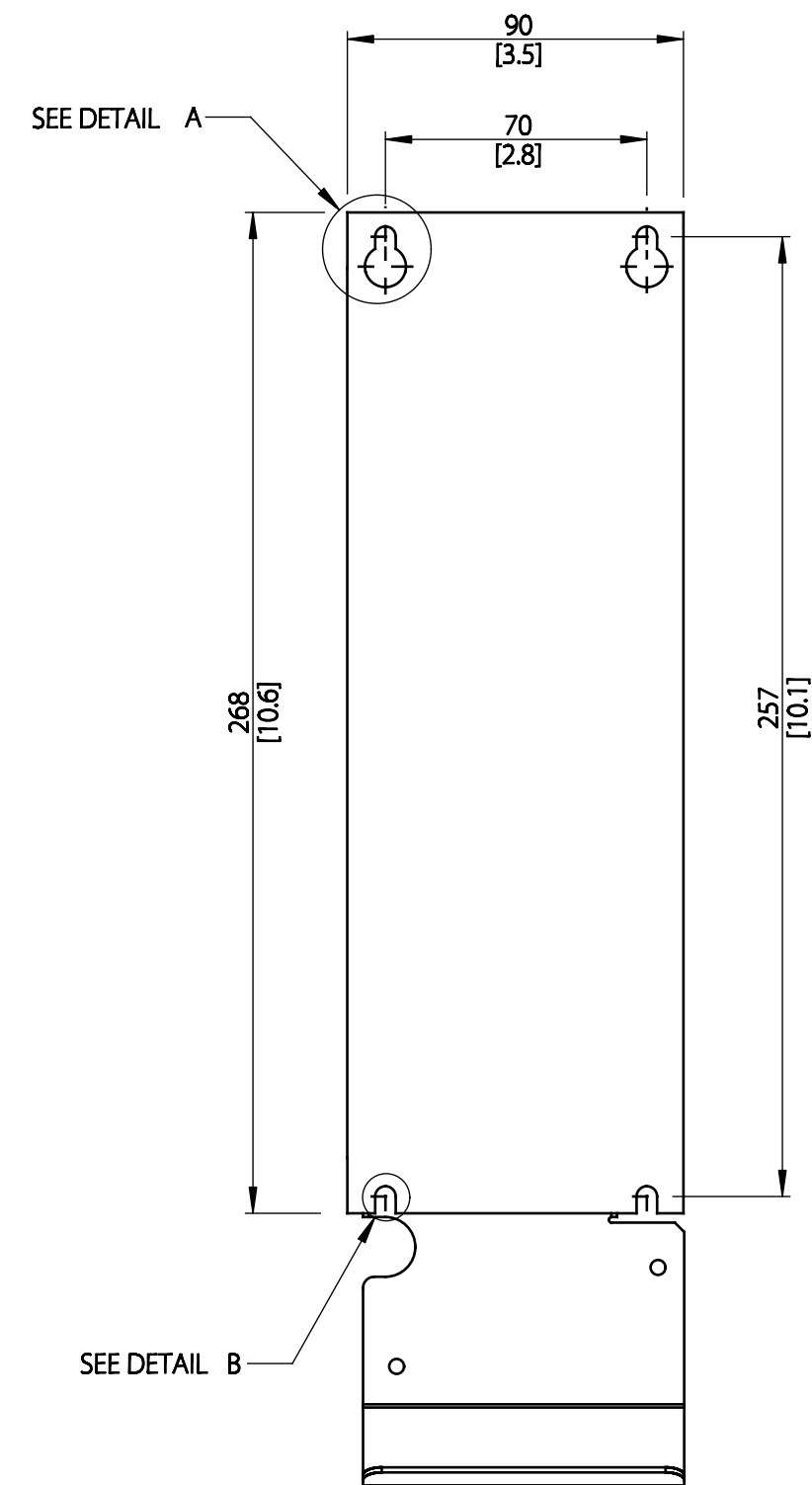
MOUNTING BASE
