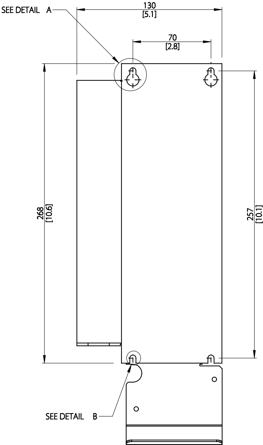
MOUNTING BASE
