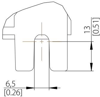
2x DETAIL B SCALE 1:1
